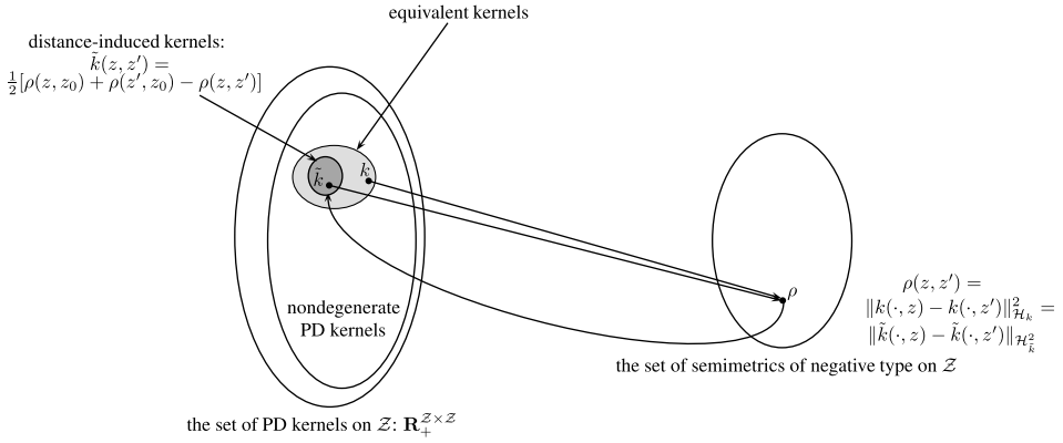
FIG. 1. The relationship between kernels and semimetrics. An equivalence class of nondegenerate PD kernels is associated to a single semimetric of negative type, and distance kernels induced by that semimetric form only a subset of that class.
